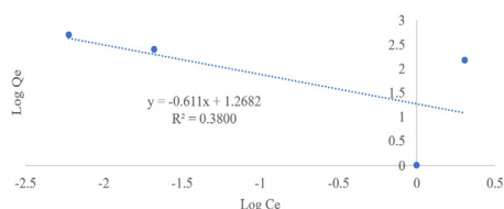
Fig. 8j: Freundlich isotherm for adsorption of Cd vs Pb vs Hg in ternary aqueous solution onto SB350 (solution volume: 100 ml; adsorbent dose: 2, 4, 8 and 10 g; contact time: 60 min)
