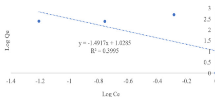
Fig. 8c: Freundlich isotherm for adsorption of Cd vs Pb vs Hg in ternary aqueous solution onto GS350 (solution volume: 100 ml; adsorbent dose: 2, 4, 8 and 10 g; contact time: 60 min)
