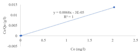
Fig. 7j: Langmuir isotherm for adsorption of Cd vs Pb vs Hg in ternary aqueous solution onto SB350 (solution volume: 100 ml; adsorbent dose: 2, 4, 8 and 10 g; contact time: 60 min)
