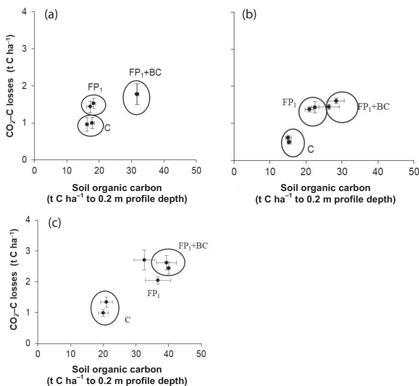
Figure 4: Relationship between soil carbon and CO 2 -C losses in Ouagadougou (Burkina Faso) during (a) crop 1 (b) crop 4, and (c) crop 11. Data show mean ( n = 4 ) \pm one standard error, during a multi-factorial cropping experiment conducted from May 2014 to April 2016. Soil carbon was calculated per m 2 to a depth of 0.2 m. Circles drawn around treatments do not represent any statistical analysis but highlight the dynamics between treatments over time.
