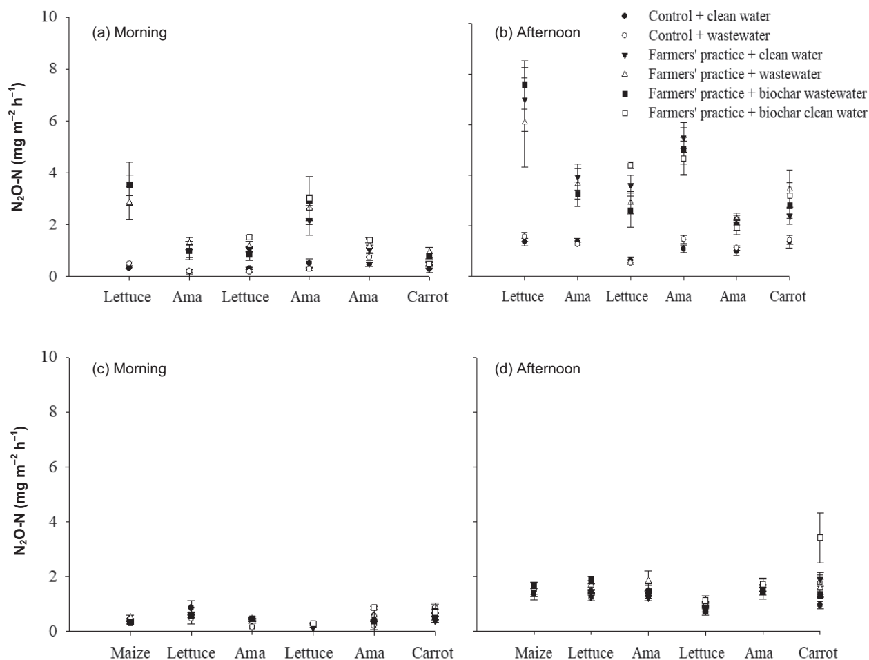
Figure 1: Effects of time of the day on emission rates of N_2O-N in (a, b) Ouagadougou, Burkina Faso and (c, d) Tamale, Ghana. Data points are means of all measurements carried out during each cycle \pm one standard error, in a multi-factorial cropping experiment conducted from May 2014 to April 2016. Ama = amaranth.
