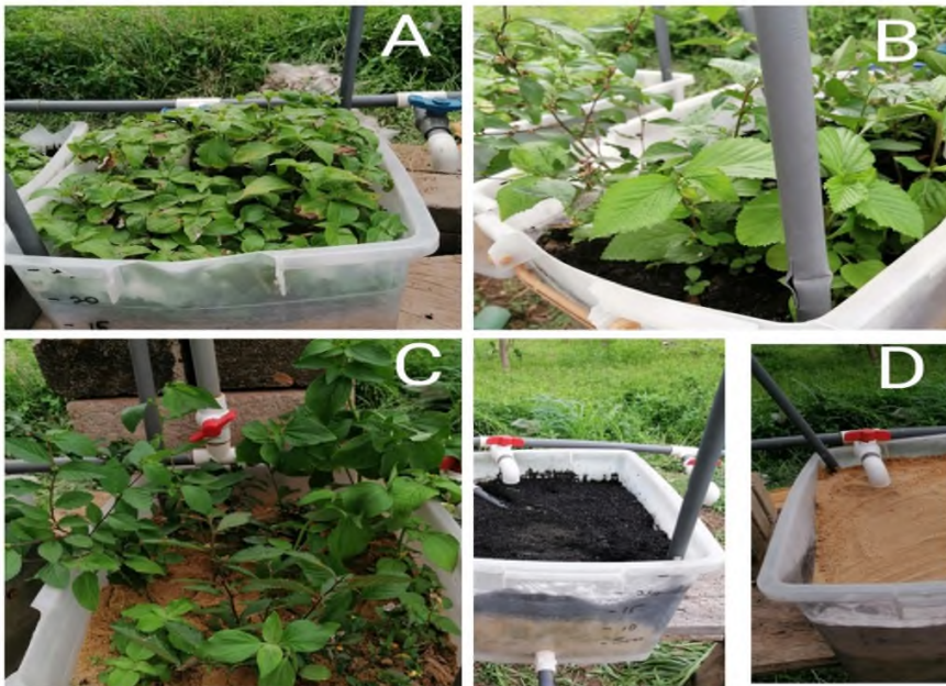
Figure 5: Experimental set up of the vertical flow CW with planted macrophytes
