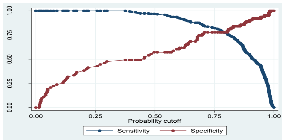
Figure 7: Probability Cutoff Graph
